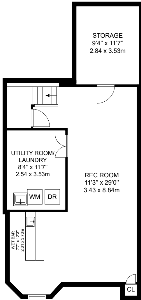
LOWER LEVEL
