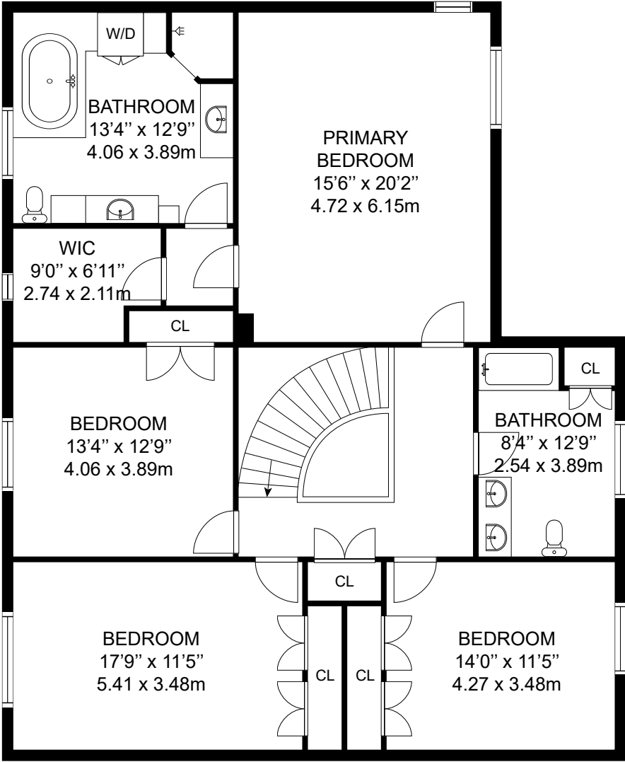
2ND LEVEL
