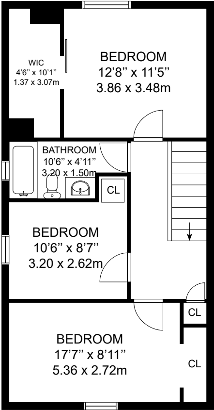
2ND LEVEL
