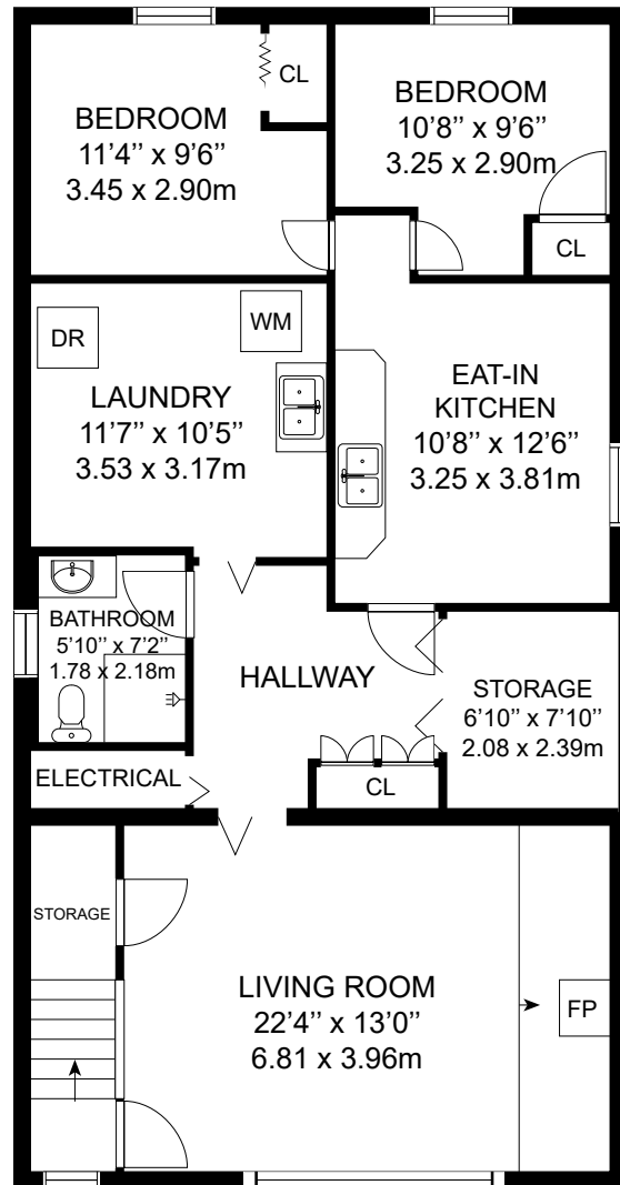
LOWER LEVEL
