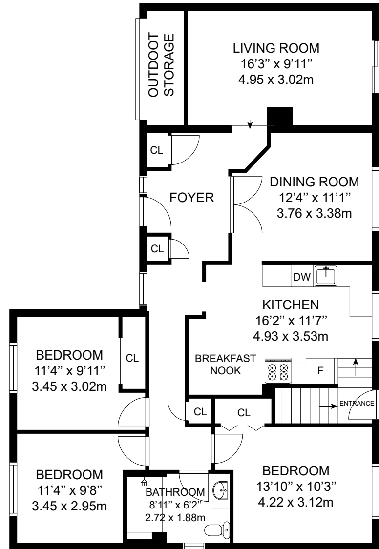
MAIN LEVEL
