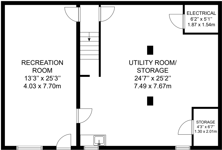
BASEMENT
