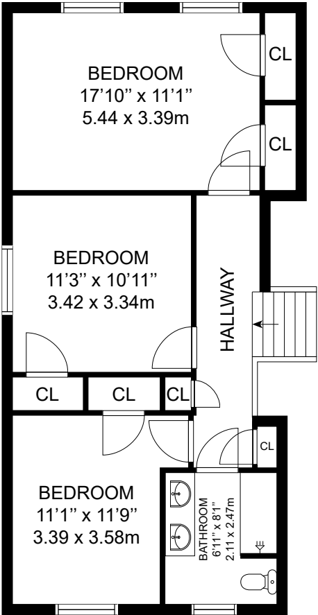
2ND FLOOR
