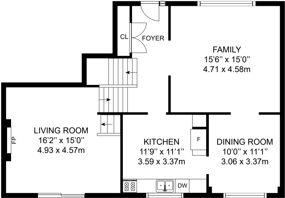
MAIN FLOOR
