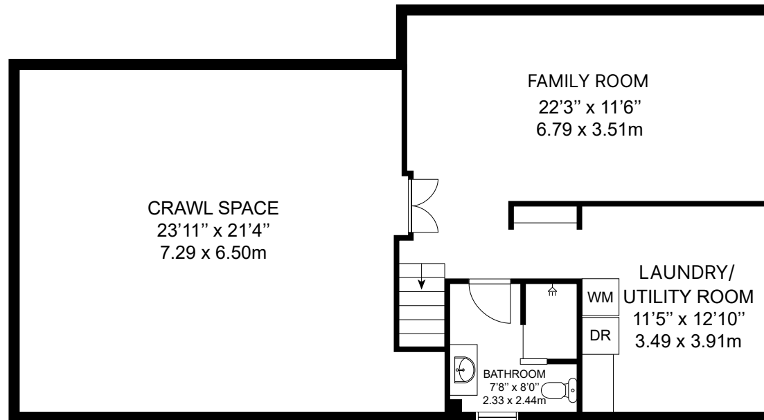
BASEMENT
