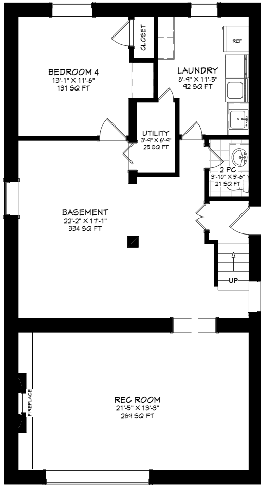
LOWER LEVEL LIVING AREA 1156 SQ FT
